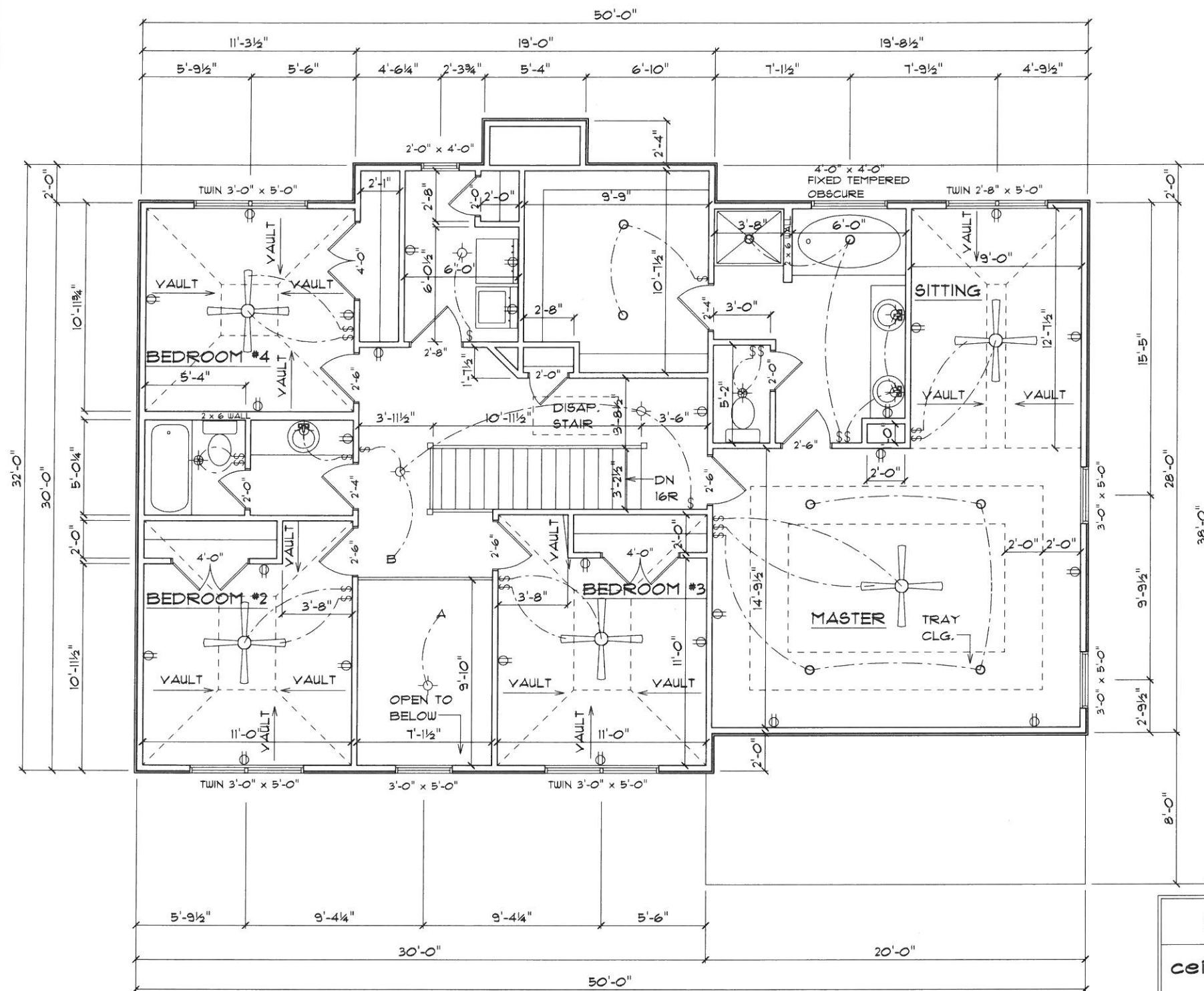
2ND FLOOR PLAN SCALE: 1/4" = 1'-0"
